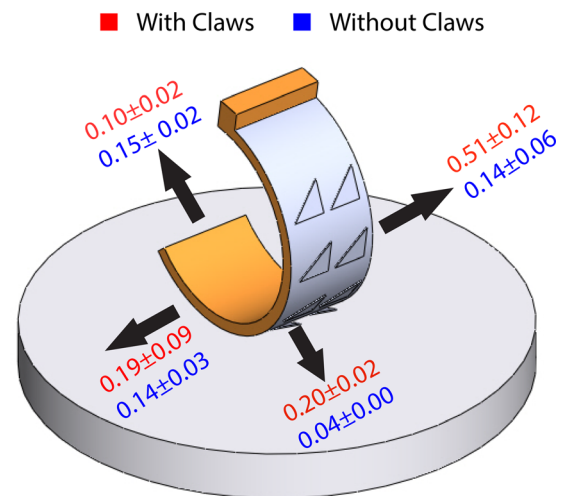
Fig. 23 The forces required to disengage the spines from a piece of corkboard. The arrows indicate the disengagement force's direction.
