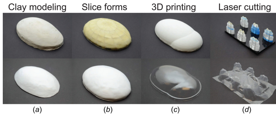
Fig. 12 Top: molds constructed using (a) clay modeling, (b) slice forms, (c) 3D printing, and (d) laser cutting. Bottom: exoskeleton shells made from these molds by thermoforming using ((a) and (b)) 750 \mu\text{m} polystyrene, (c) 250 \mu\text{m} polycarbonate, and (d) 50 \mu\text{m} polyethylene.
