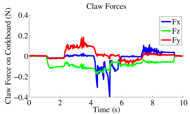
Fig. 22 Plot of the forces exerted by the claw onto a test substrate as it is pulled in the F_x and F_y directions and preloaded with F_z . F_z , F_y indicates the fore-aft forces while F_x shows lateral forces.
